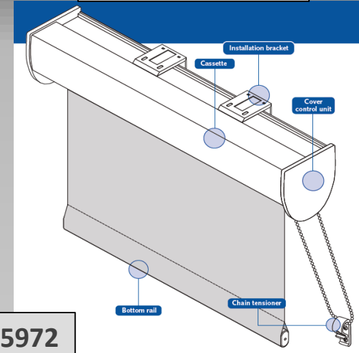
V53-Roller blind PL-5353
